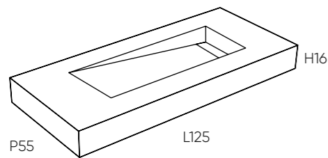
Sanitarni pult sa integriranim kosim umivaonikom: INFINITY Integrated top with degrade washbasin: INFINITY
