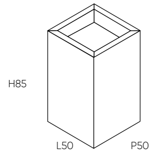
Samostojeći sanitarni pult: KUBE Pedestal mounted washbasin: KUBE
